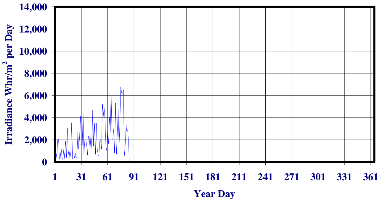
Eugene, Or. 1998 Daily Irradiance on 60 Degree Tilt Facing South
