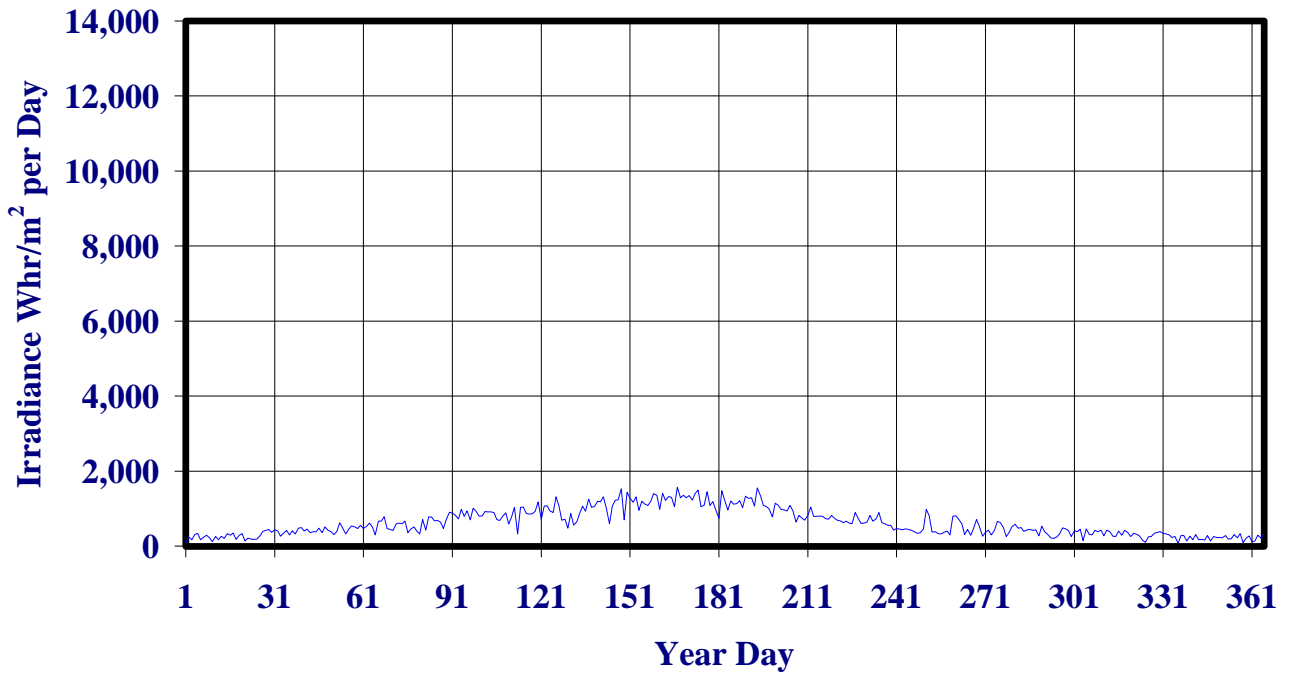
Eugene, Or. 1998 Daily Irradiance on 90 Degree Tilt Facing North
