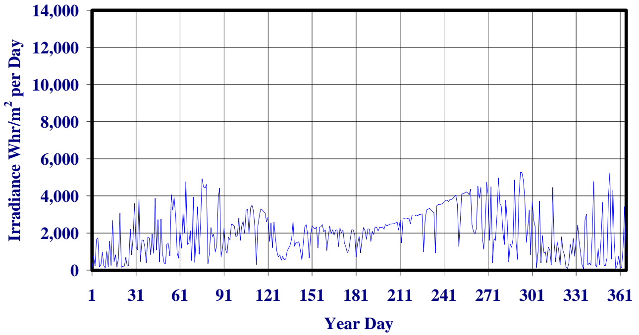
Eugene, Or. 1998 Daily Irradiance on 90 Degree Tilt Facing South
