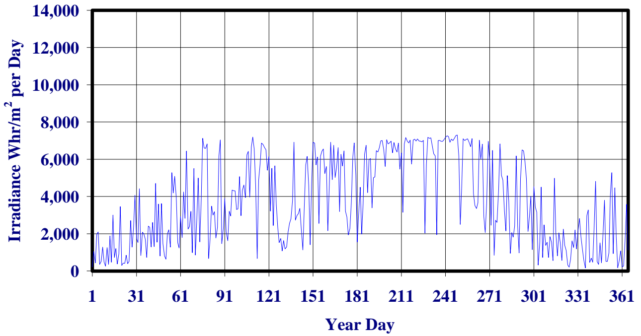
Eugene, Or. 1998 Daily Irradiance on 45 Degree Tilt Facing South
